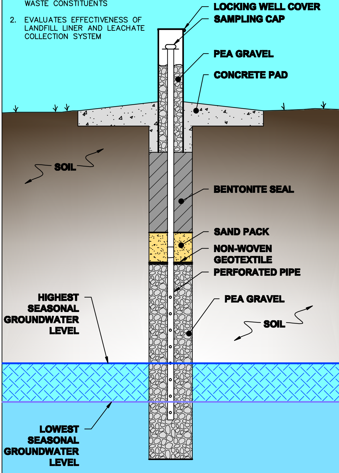
TYPICAL GROUNDWATER MONITORING WELL
